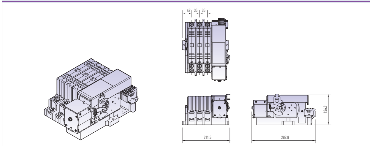
ATS-F TYPE [100A~200A] 4P 100AF
