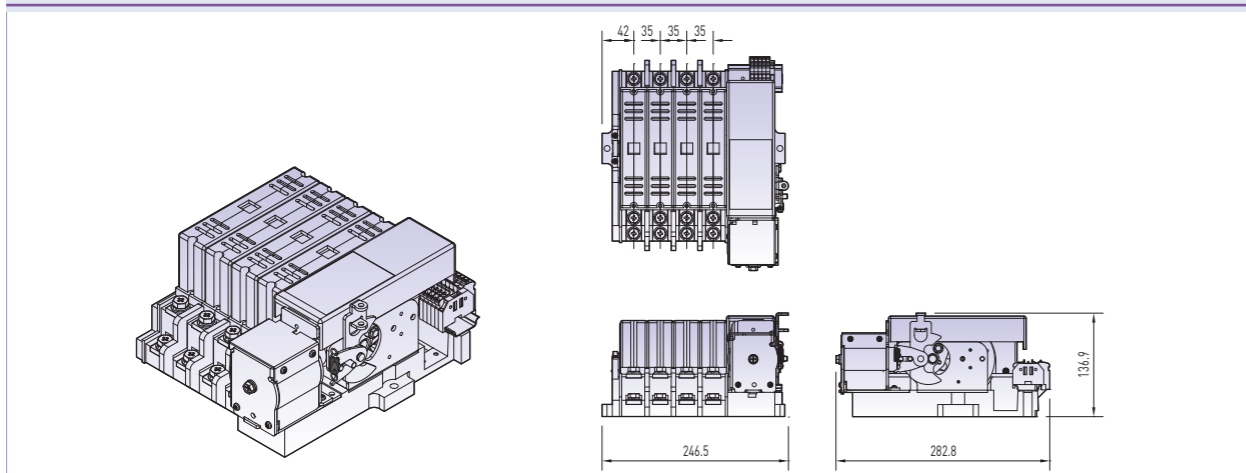
ATS-F TYPE [100A~200A] 4P 100AF
