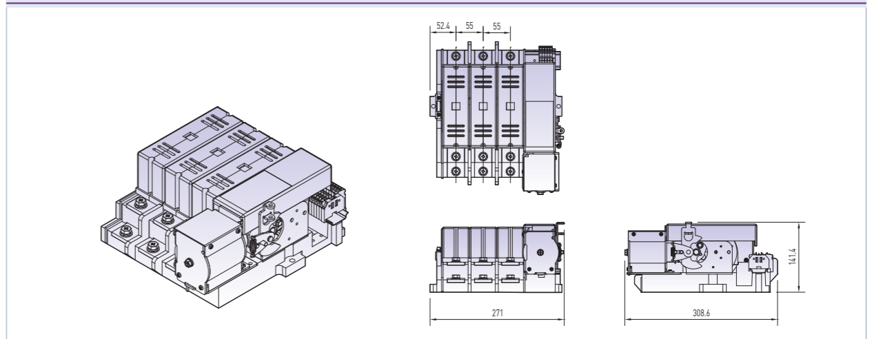
ATS-F TYPE [400A~600A] 4P 400AF
