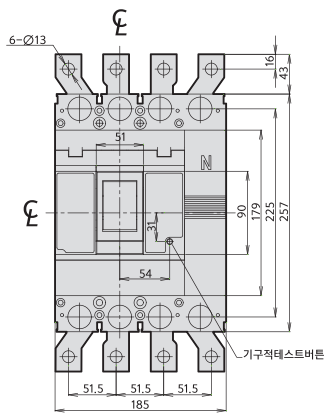
4Pole
